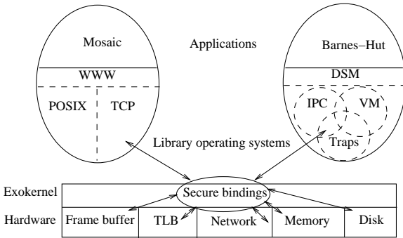
Figure 1: An example exokernel-based system consisting of a thin exokernel veneer that exports resources to library operating systems through secure bindings. Each library operating system implements its own system objects and policies. Applications link against standard libraries (e.g., WWW, POSIX, and TCP libraries for Web applications) or against specialized libraries (e.g., a distributed shared memory library for parallel applications).
